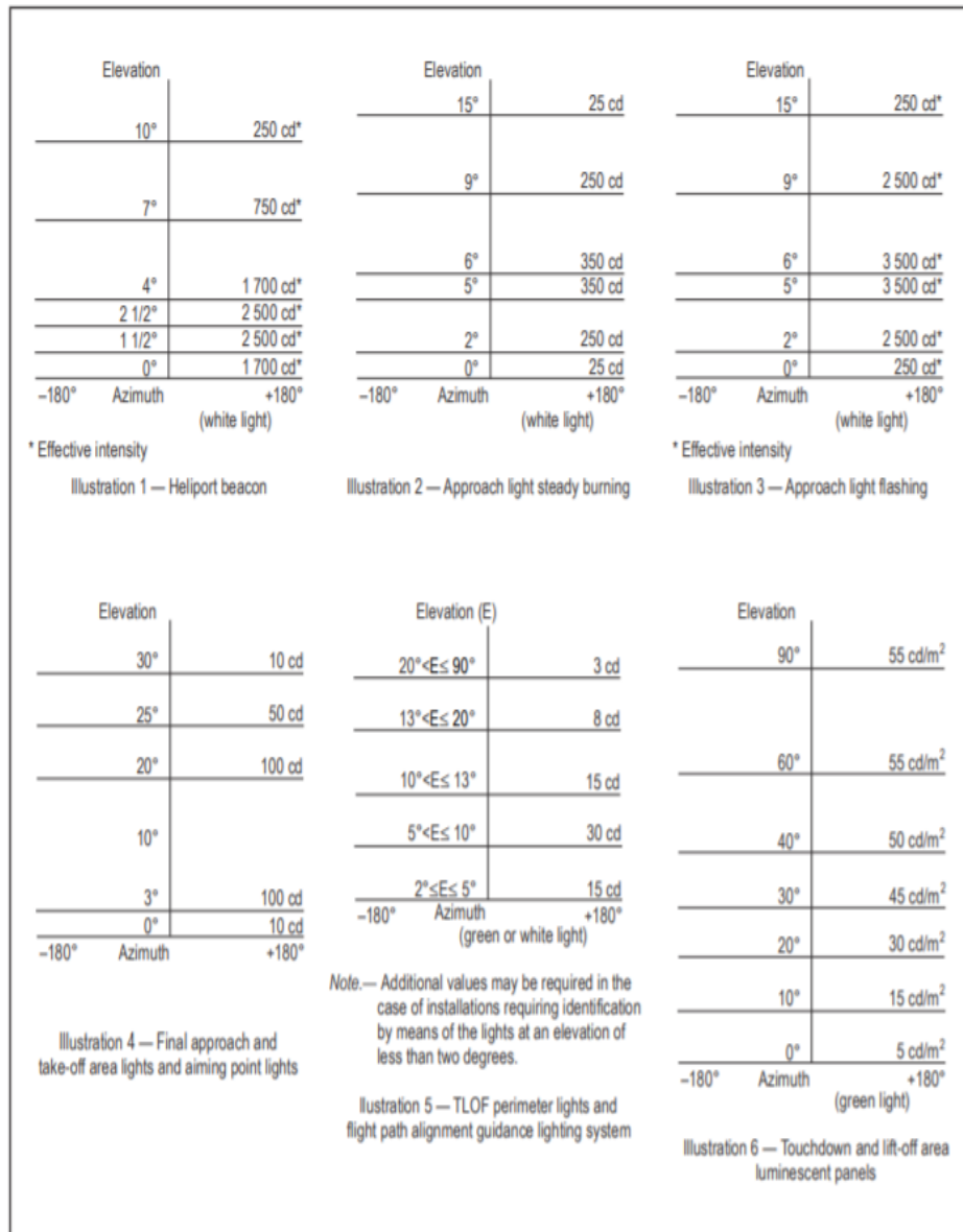
Figure 4-12. Isocandela diagrams
