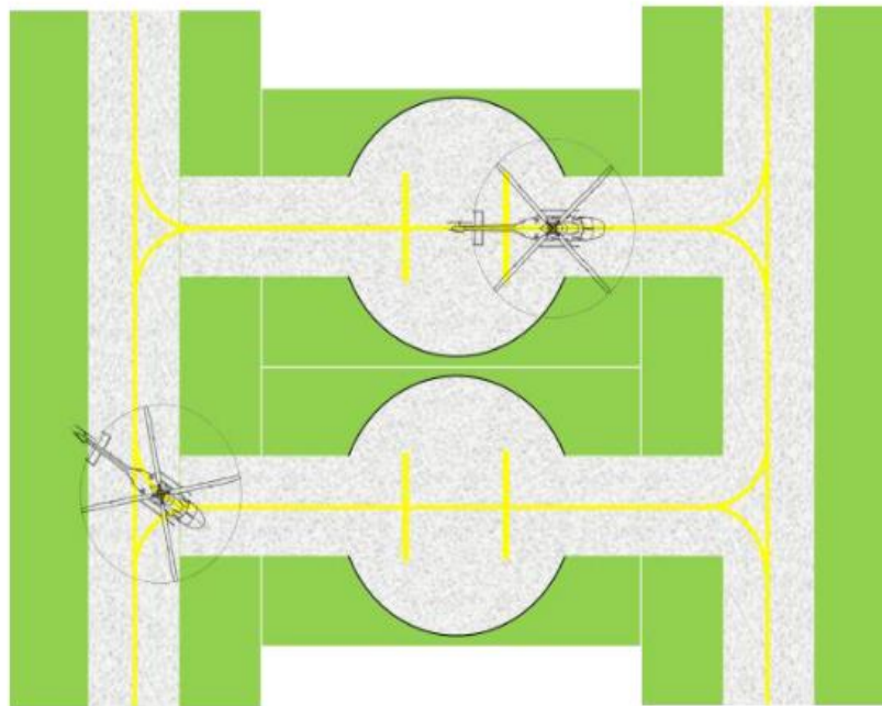
Figure 2-6. Ground taxi-through stands (with taxiway/ground taxi-route) simultaneous use
