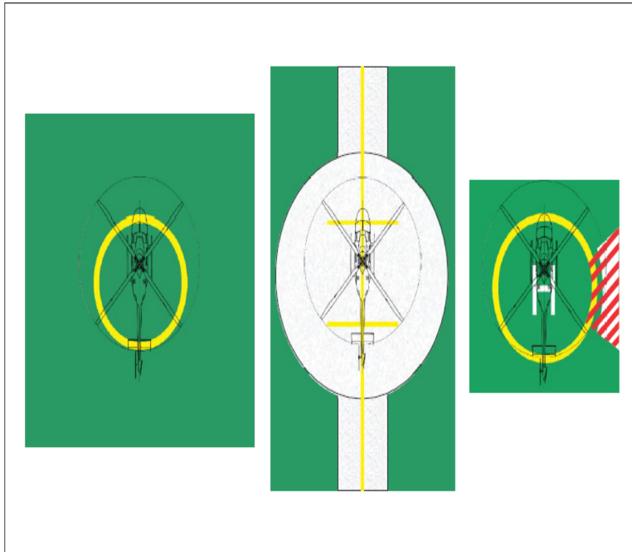
Figure 5-8. Multidirectional TDPC with no limitations (left) Unidirectional marking shoulder line with associated centreline (centre) Multidirectional TDPC with prohibited landing sector marking (right)
