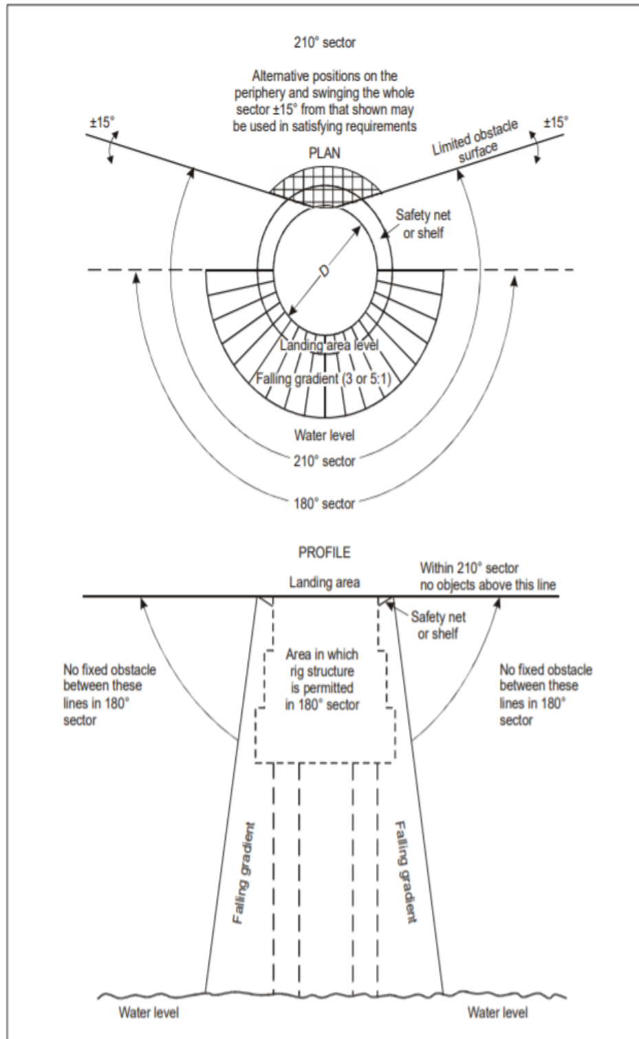
Figure 3-7. Helideck obstacle-free sector
