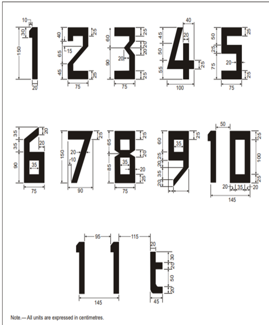
Figure 4-5. Form and proportions of numbers and letters
