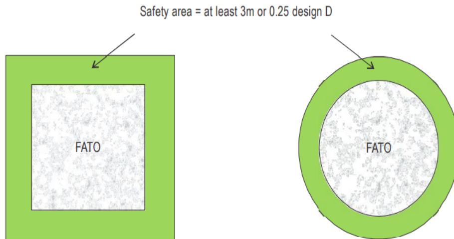
Figure 2-1. FATO and associated safety area
