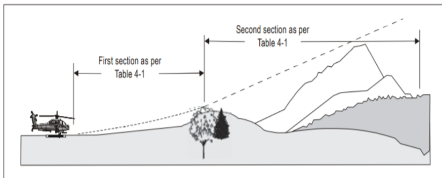
b) Approach and take-off climb surfaces - "B" slope profile - 8% and 16% design
