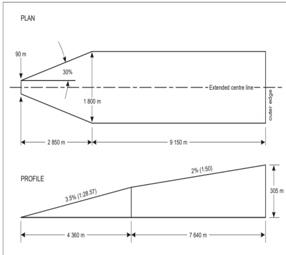
Figure S-2. Take-off climb surface for instrument FATO
