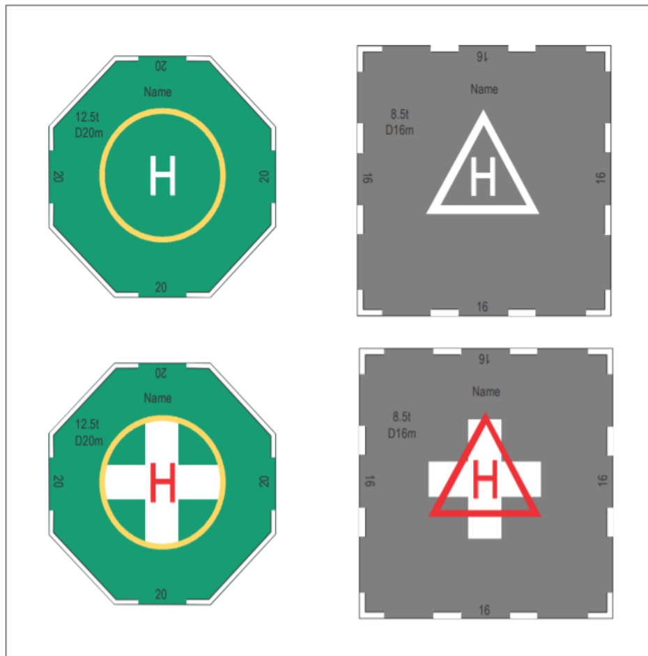
Figure Figure 4-2. Heliport identification markings with TLOF and aiming markings for heliport and hospital heliport
