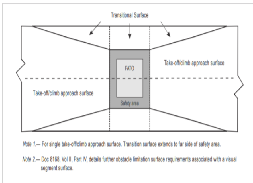
Figure S-5. Transitional surfaces for an instrument FATO with a non-precision or precision approach
