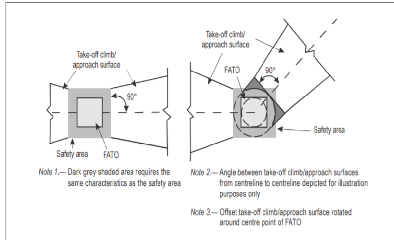
Figure 3-1. Obstacle limitation surfaces — Take-off climb and approach surface
