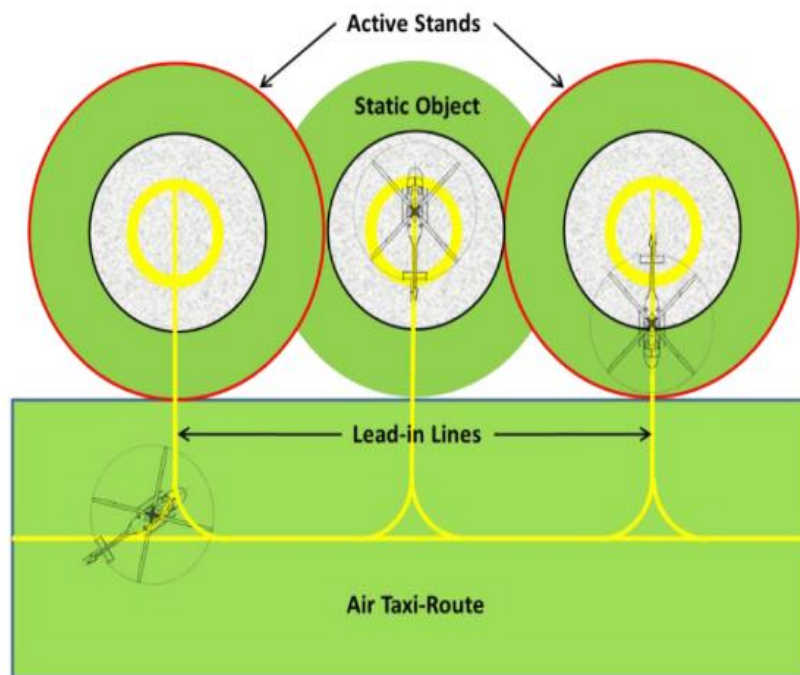
Figure 2-7. Air taxi-through stands (with air taxi-route) simultaneous use
