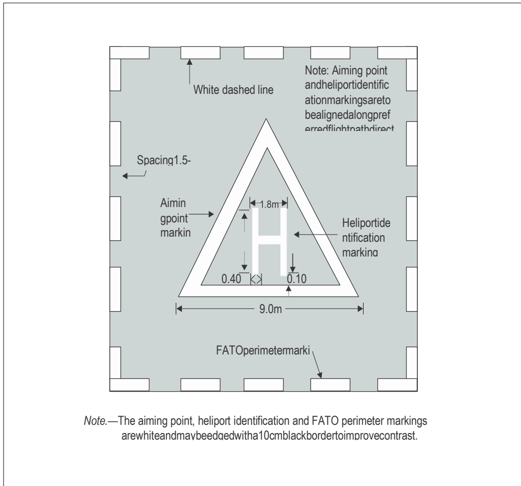
Figure 4-1. Combined heliport identification, aiming point and FATO perimeter marking
