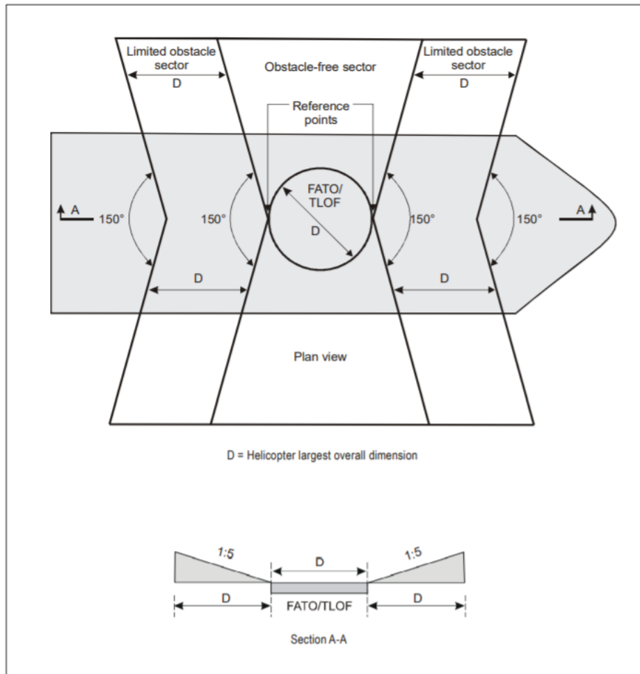
Figure 3-10. Amidship's location — shipboard heliport obstacle limitation surfaces
