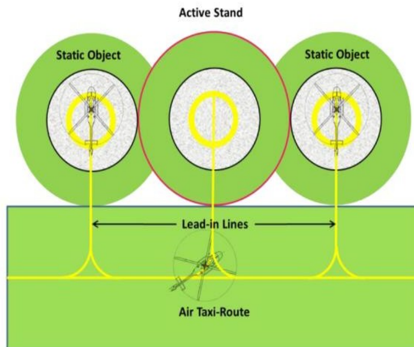
Figure 2-9. Turning stands (with air taxi-route) non-simultaneous use – inner stand active
