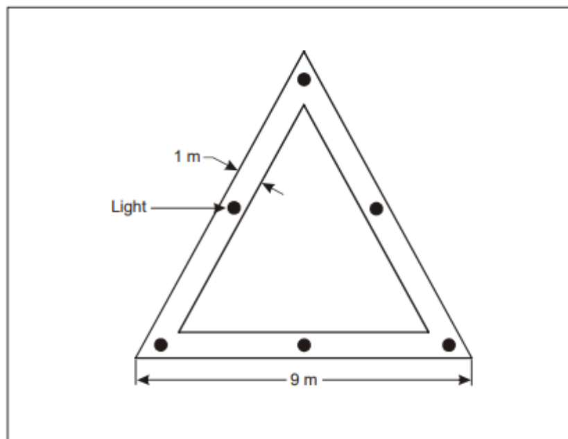
Figure 4-7. Aiming point marking
