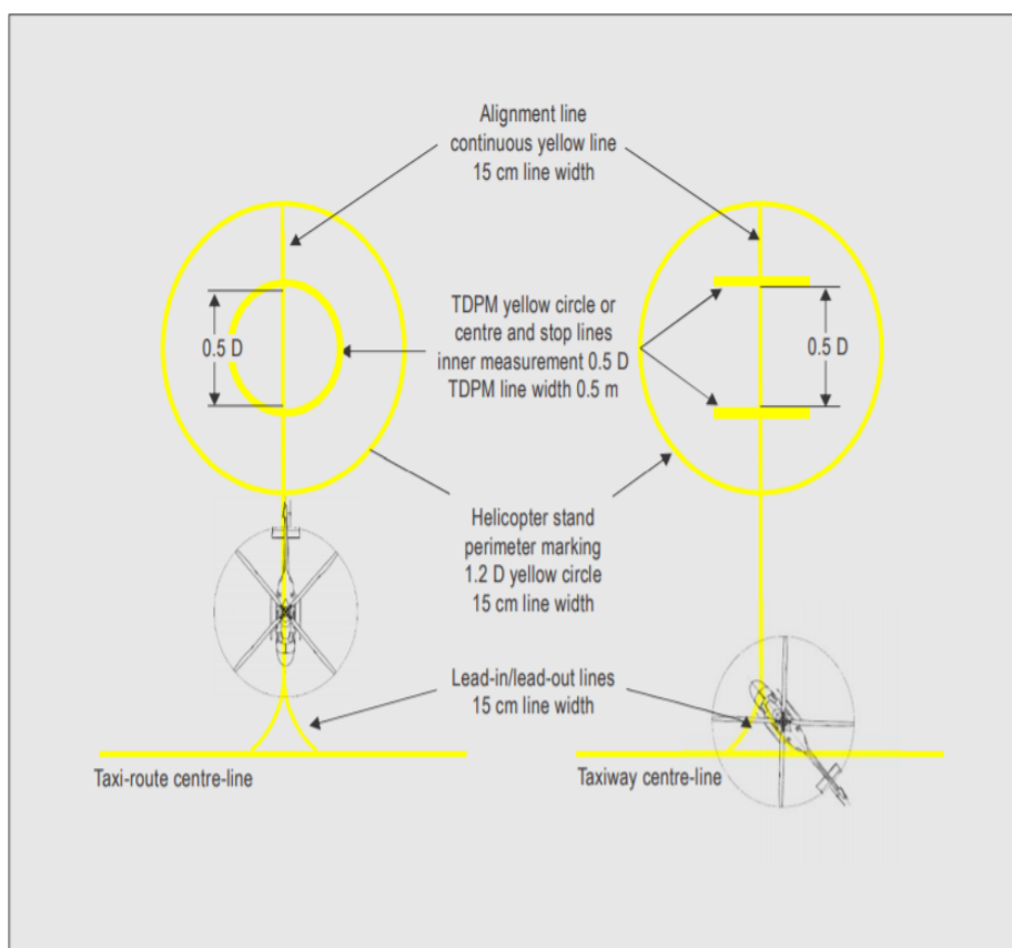
Figure 4-9. Helicopter stand markings
