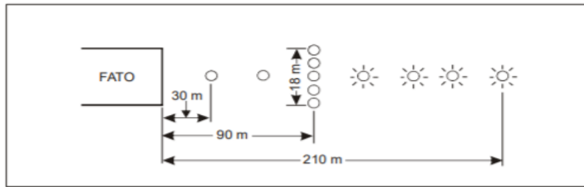
Figure 4-13. Approach lighting system
