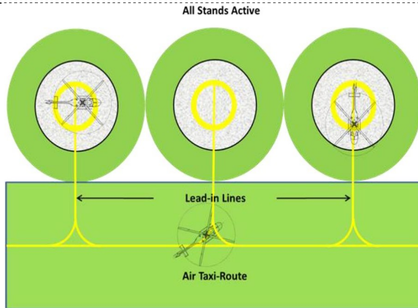
Figure 2-5. Turning stands (with air taxi-routes)— simultaneous use
