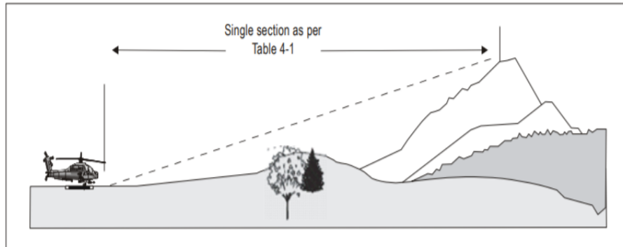
c) Approach and take-off climb surfaces - "C" slope profile - 12.5% design
