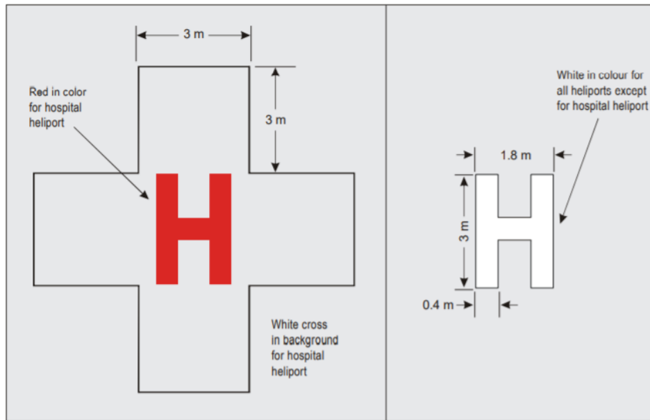
Figure 4-4. Hospital heliport identification and heliport identification marking
