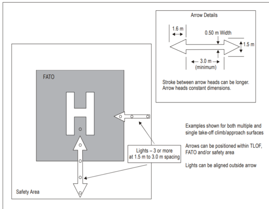
Figure 4-10. Flight path alignment guidance markings and lights
