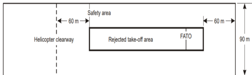
Figure S-1. Safety Area for Instrument FATO
