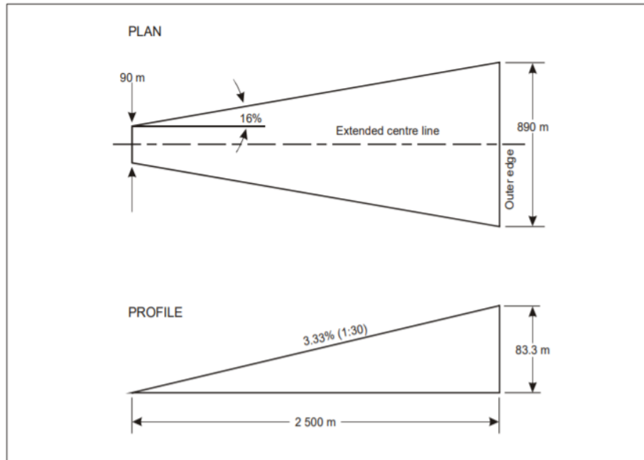
Figure S-4. Approach Surface for non-precision approach FATO
