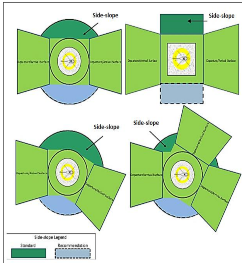
Figure 2-2. FATO simple/complex safety area and side slope protection
