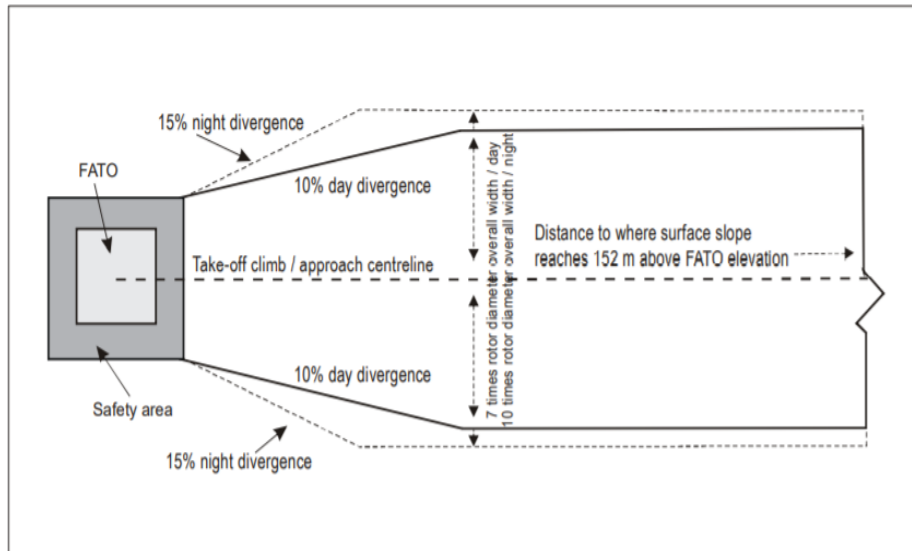
Figure 3-2. Take-off climb/Approach surface width
