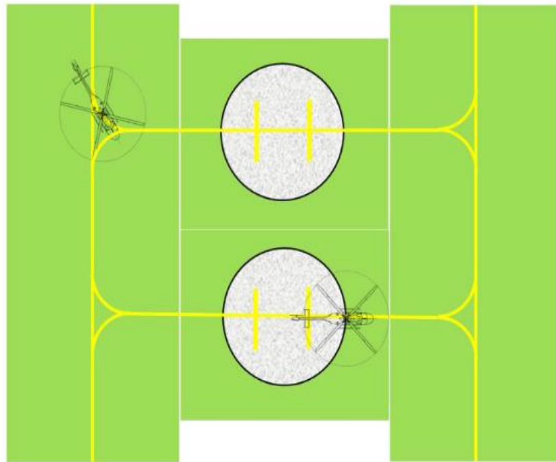
Figure 2-7. Air taxi-through stands (with air taxi-route) simultaneous use
