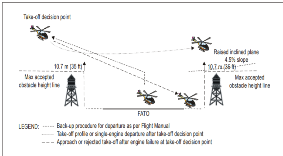
Figure 3-4. Example of raised inclined plane during operations in performance Class 1
