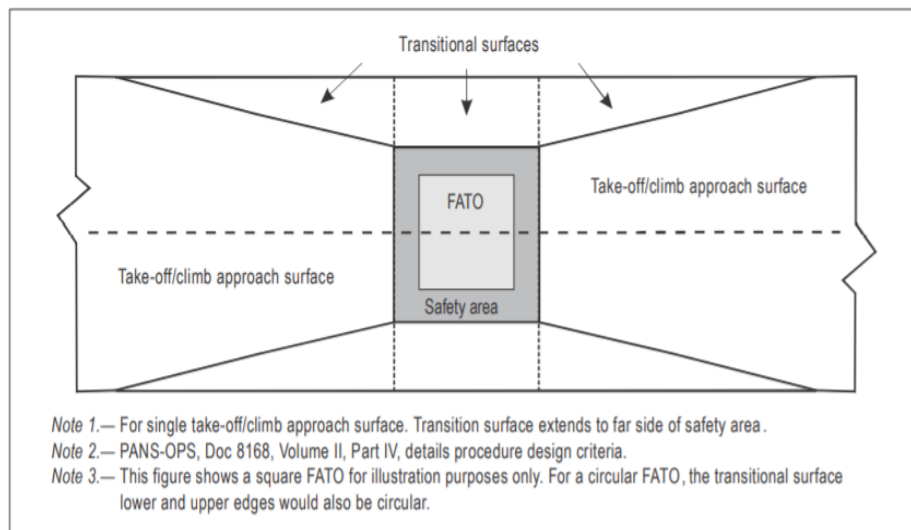
Figure 3-3. Transitional surface for a FATO with a PinS approach procedure with a VSS
