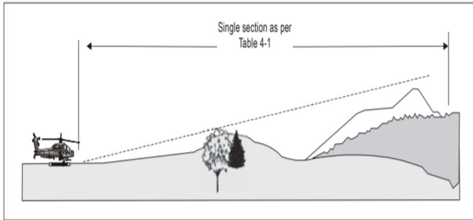
a) Approach and take-off climb surfaces - "A" slope profile - 4.5% design
